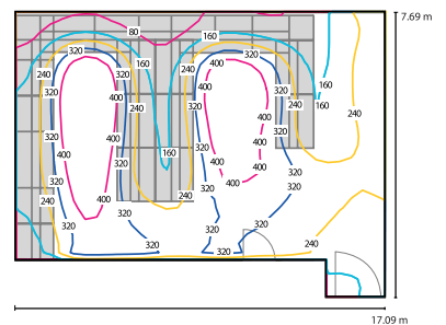
Light planning (isolines showing the illumination values in lux at every point in the room)
