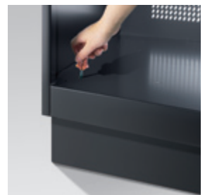
Base can be height adjusted from inside: For easier adjustment of individual lockers and locker rows.
